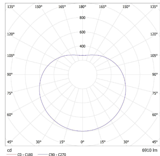
Lucis ZK.P4.500.X POLARIS ZK LED / LDC (Polar)
